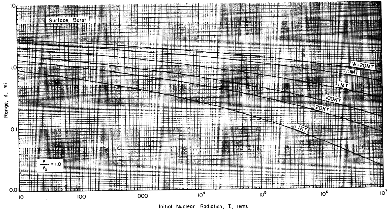
Fig. 2.17—Initial nuclear radiation as a function of range and yield for surface bursts (see Eq. 2.115).
